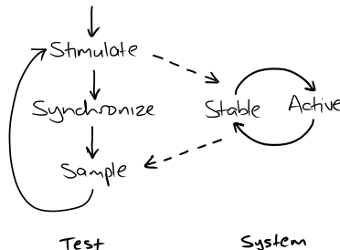
Figure 27.3 Phases of a sampling test
