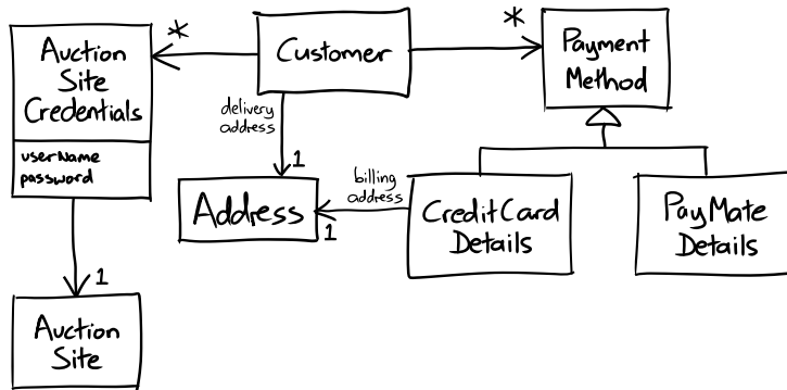
Figure 25.1 Persistent entities
