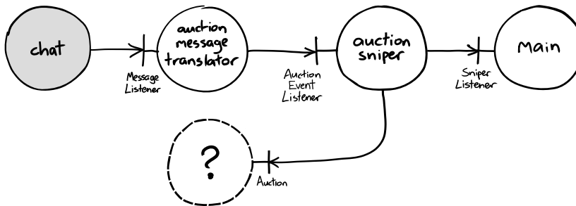
Figure 13.2 Introducing Auction
