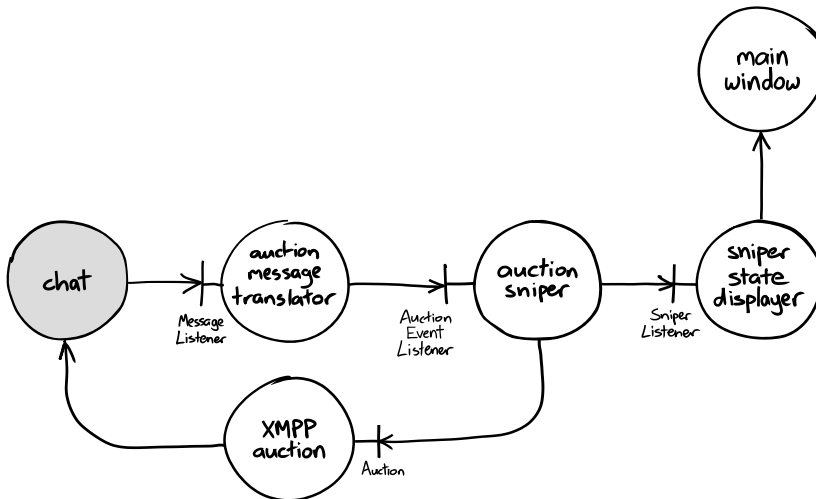
Figure 13.5 Extracting SniperStateDisplayer
